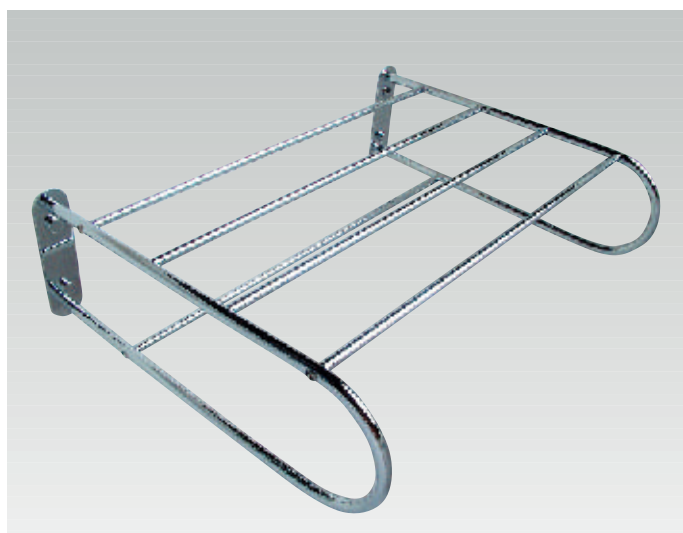
P-24 Toallero repisa 47x35x14 cm. P-24 Towel shelf 47x35x14 cm.
